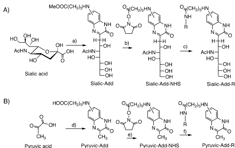
Scheme 4. Preparation of the quinoxalinone adducts of sialic acid (A) and pyruvic acid (B) and their elaboration into the NHS esters, and either the BSA conjugates ( \text{R} = \text{BSA} ) or affinity supports ( \text{R} = \text{sepharose} ). a) \text{Na}_2\text{S}_2\text{O}_4 , diamine, \text{AcOH}/\text{H}_2\text{O} (9:1), 50 °C, 2 h, 52 %; b) 1. \text{NaOH} (0.03 M), 97 %; 2. TSTU, dioxane/DMF/ \text{H}_2\text{O} (2:2:1), RT, 16 h, 42 %; c) BSA or amino-sepharose, phosphate buffer (0.1 M, pH 7.1), \text{H}_2\text{O} , RT, 16 h; d) 1. (see Scheme 3) with diamine, \text{HCl} (0.5 M), 50 °C, 1 h; 2. \text{NaOH} (0.03 M), RT, 30 min, 68 % (over two steps); e) EDC, NHS, DMF, RT, 16 h, 37 %; f) (see Scheme 3) with BSA or amino-sepharose, \text{H}_2\text{O}/\text{dioxane} (10:1), RT, on. EDC = 1-ethyl-3-[3-(dimethylamino)propyl]carbodiimide hydrochloride, NHS = N -hydroxysuccinimide.
